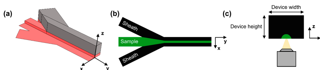
Figure 1. (a) Lengthwise 3D device cross-section showing the difference in height between the sheath and sample inlets. Red color is used to show the bottom layer of photoresist, and also the device footprint. The top layer of photoresist is shown in grey (mirror symmetry across the y-axis applies). The difference in height between the sheath inlet and the sample inlet shown is not drawn to scale and only serves as an example; (b) Device top view showing the flow focusing mechanism, where the black area is occupied by sheath fluid and the green area is occupied by the sample; (c) 2D lengthwise cross-section of the channel (front view) showing sample confinement from both the top and the sides.
